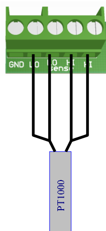
4-wire RTD connection
