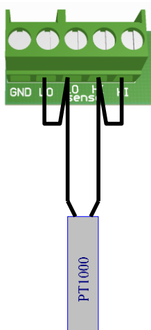
2-wire RTD connection
