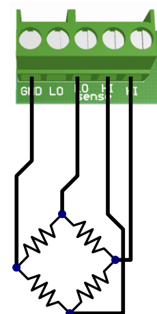
Bridge connection
